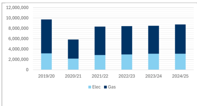
Figure 11: HDC Buildings Combined Electricity and Natural Gas kWh
